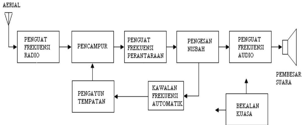
Rajah 1: Gambarajah Blok Penerima Radio FM
